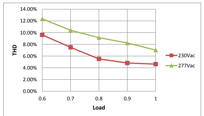
THD Curve
