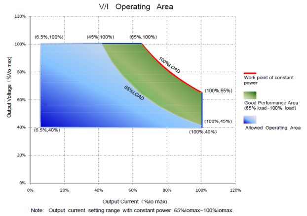
V/I Curve
