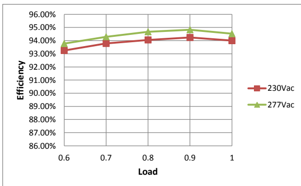
Efficiency VS. Load Curve (ME200H105AQ_CP I o =700mA typ.)
